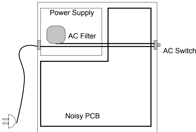
Improper ac line filter
