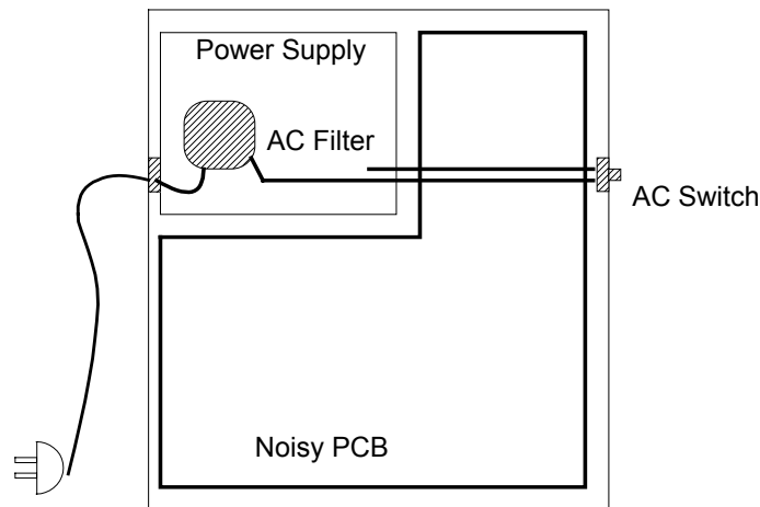
Proper ac line filter
